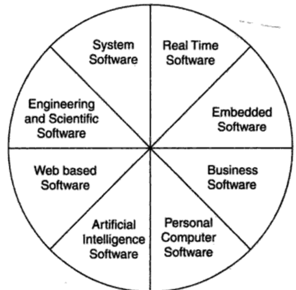
Fig. 1.7: Software applications.
