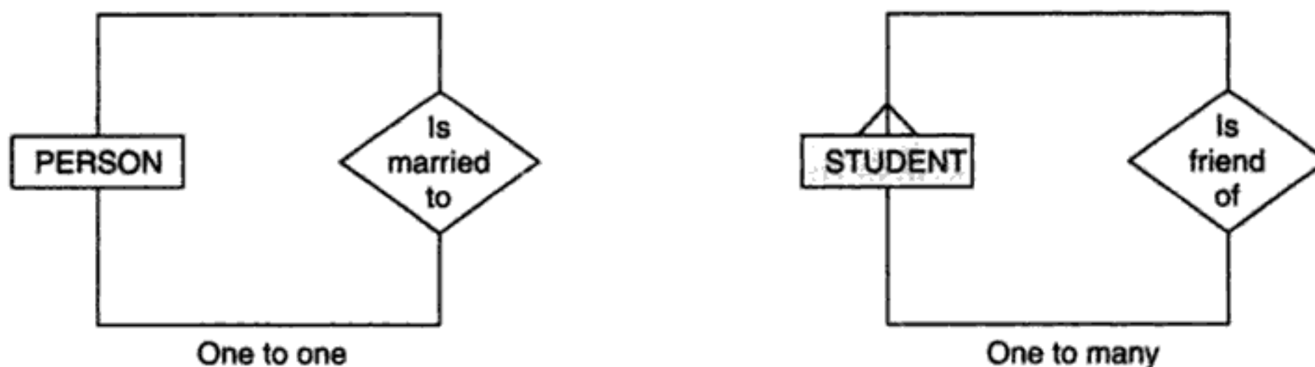
Fig. 3.12: Unary relationships.
