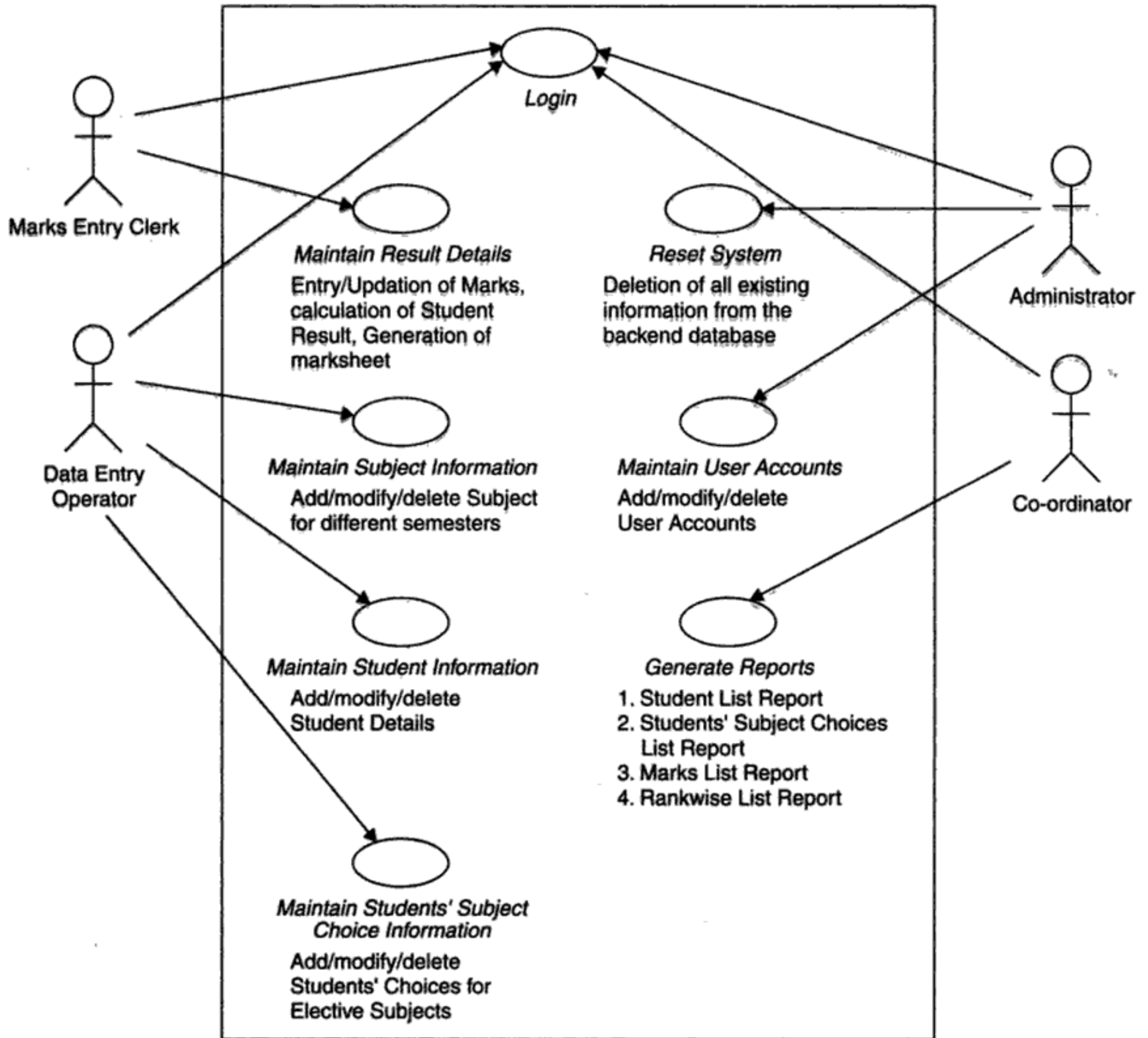
Use Case Diagram
