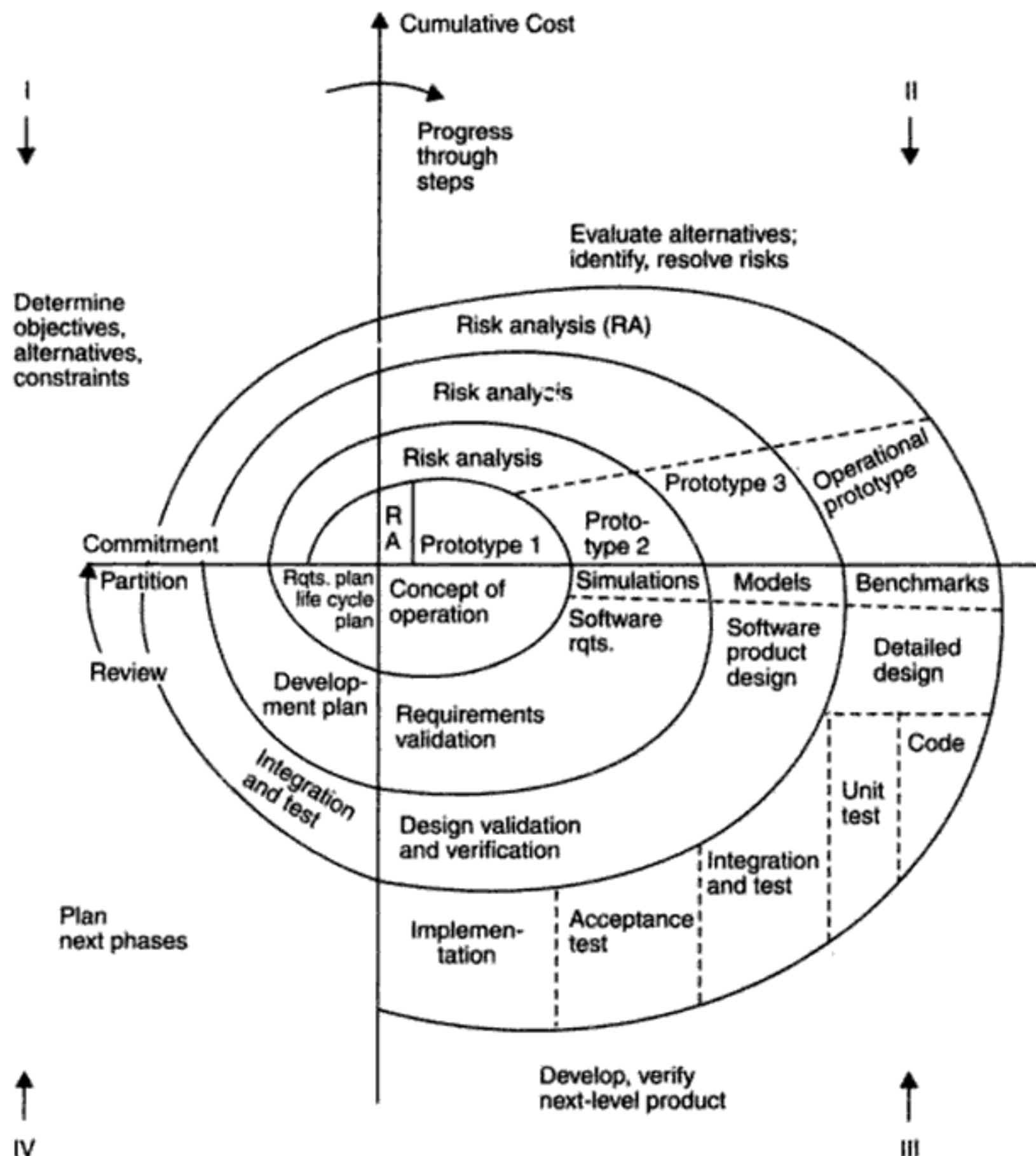
Fig. 2.5: Spiral model
