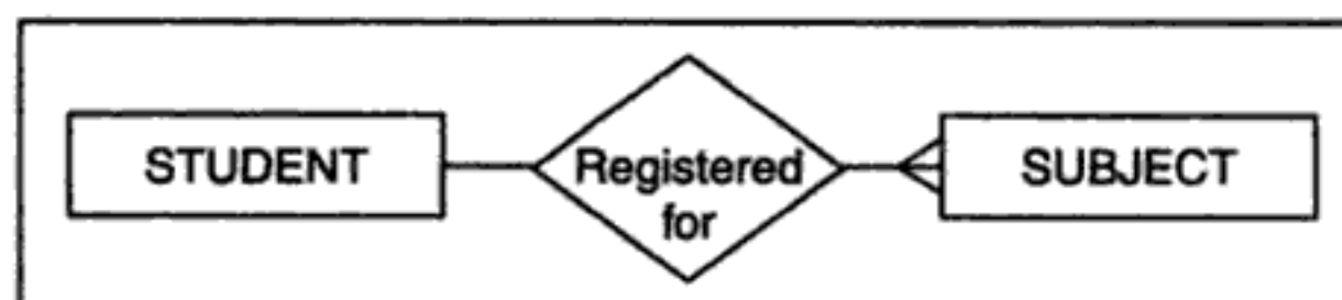
Fig. 3.15: Use of cardinality.
