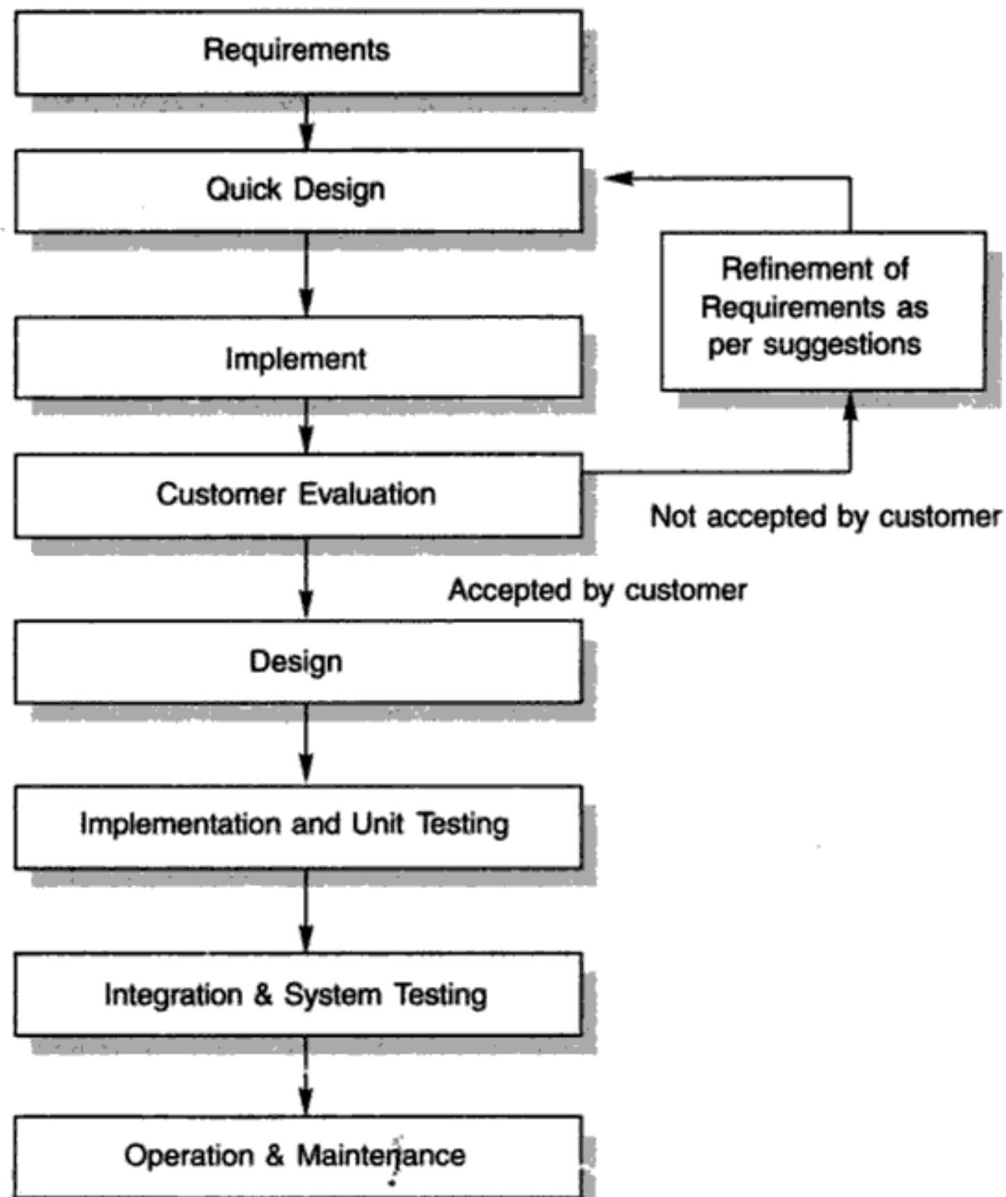
Fig. 2.3: Prototyping model
