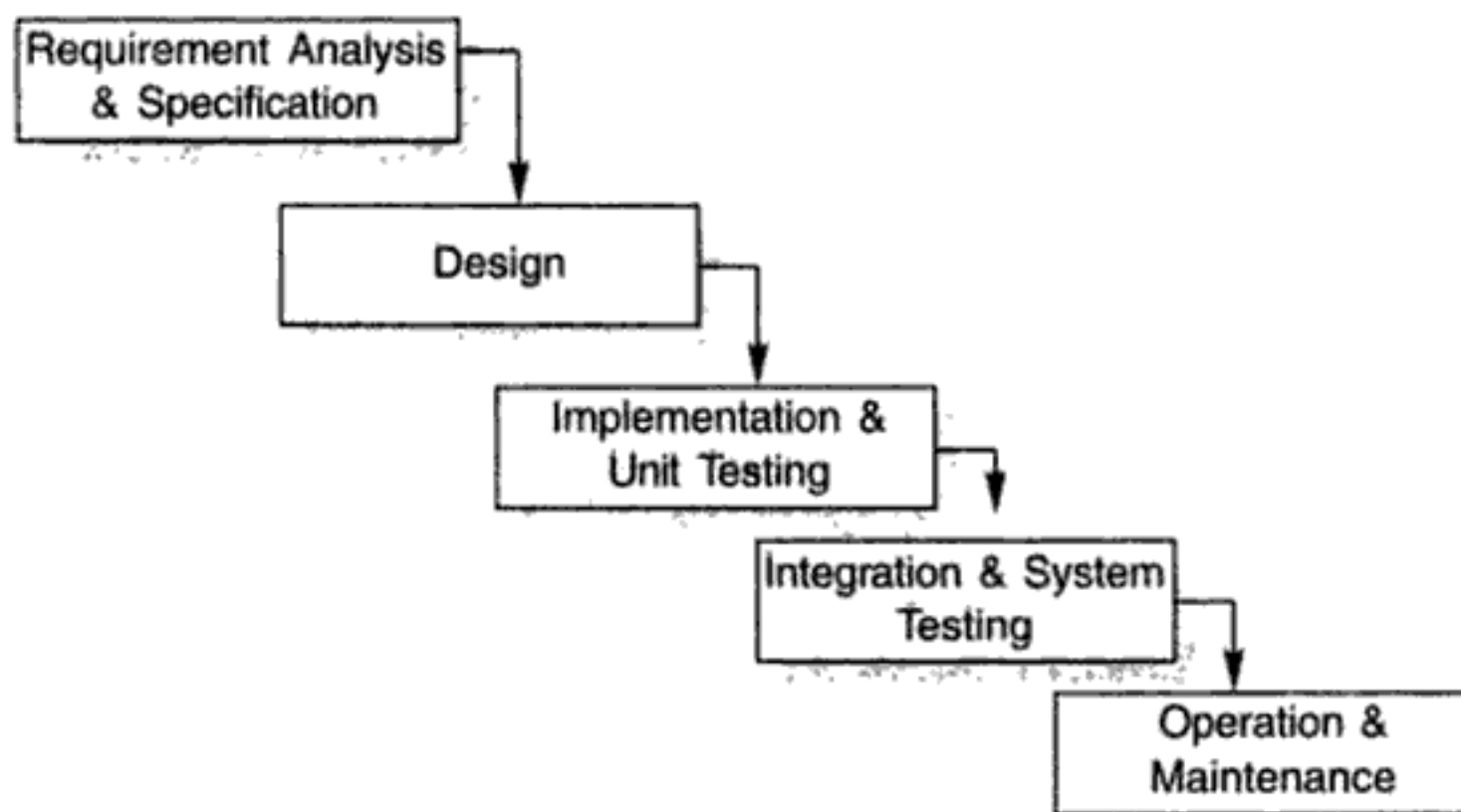
Fig. 2.2: Waterfall model
