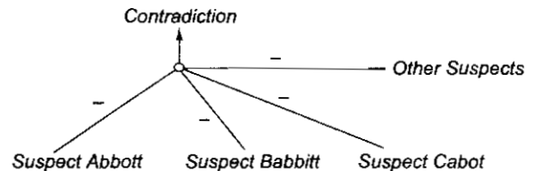
Fig. 7.10 A Contradiction
