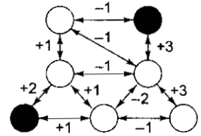
Fig. 18.1 A Simple Hopfield Network
