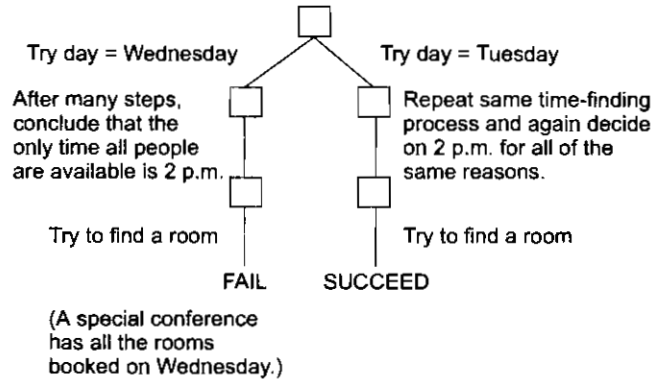
Fig. 7.4 Nondependency-Directed Backtracking
