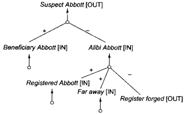
Fig. 7.7 Changed Labeling
