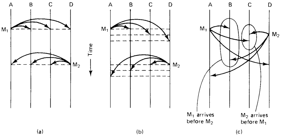
Fig. 2-37. (a) A synchronous system. (b) Loose synchrony. (c) Virtual synchrony.
