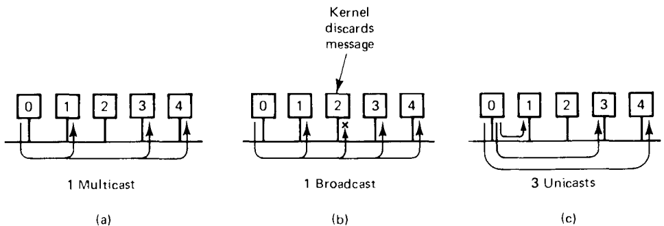
Fig. 2-33. Process 0 sending to a group consisting of processes 1, 3, and 4. (a) Multicast implementation. (b) Broadcast implementation. (c) Unicast implementation.
