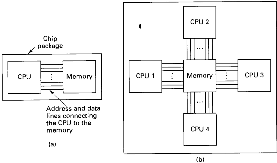
Fig. 6-1. (a) A single-chip computer. (b) A hypothetical shared-memory multiprocessor.
