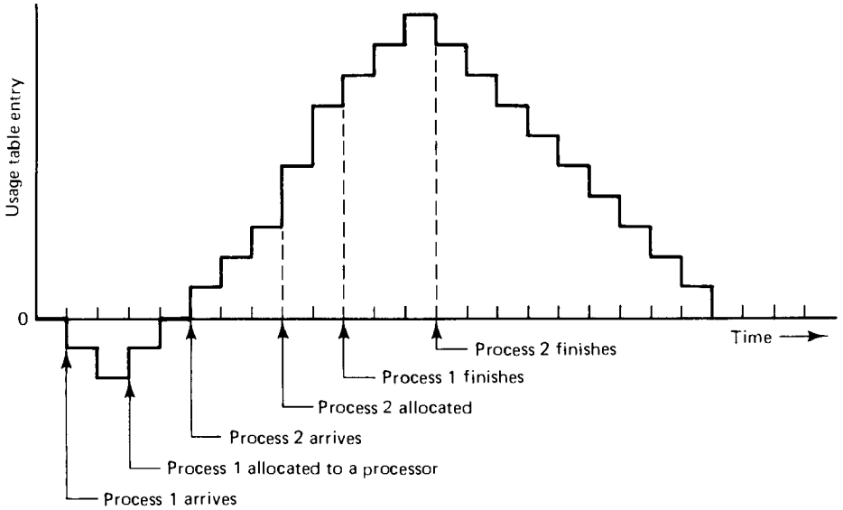
Fig. 4-18. Operation of the up-down algorithm.
