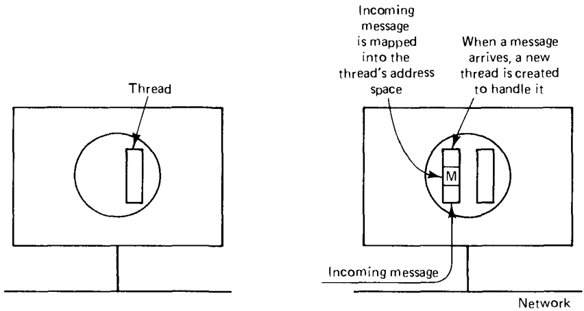
Fig. 4-9. Creating a thread when a message arrives.
