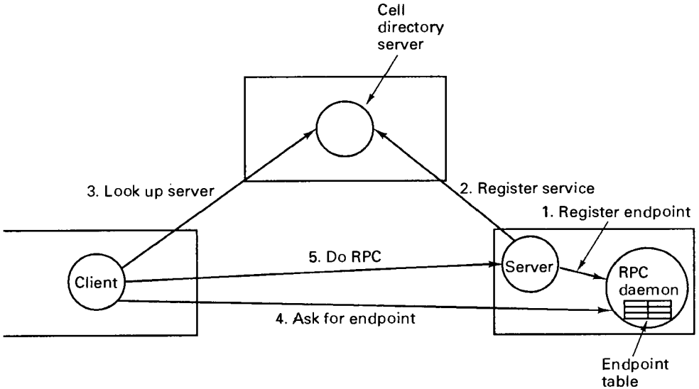
Fig. 10-14. Client-to-server binding in DCE.
