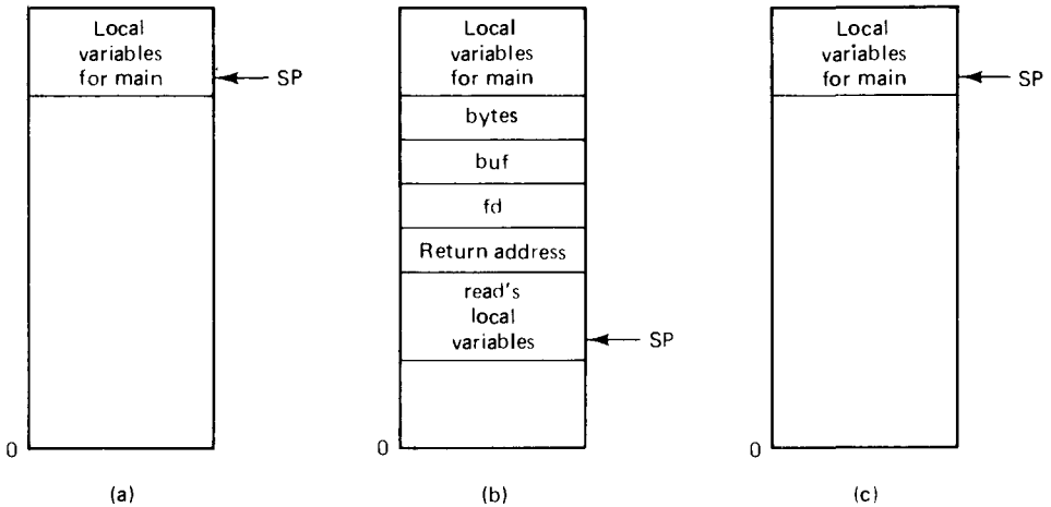
Fig. 2-17. (a) The stack before the call to read . (b) The stack while the called procedure is active. (c) The stack after the return to the caller.
