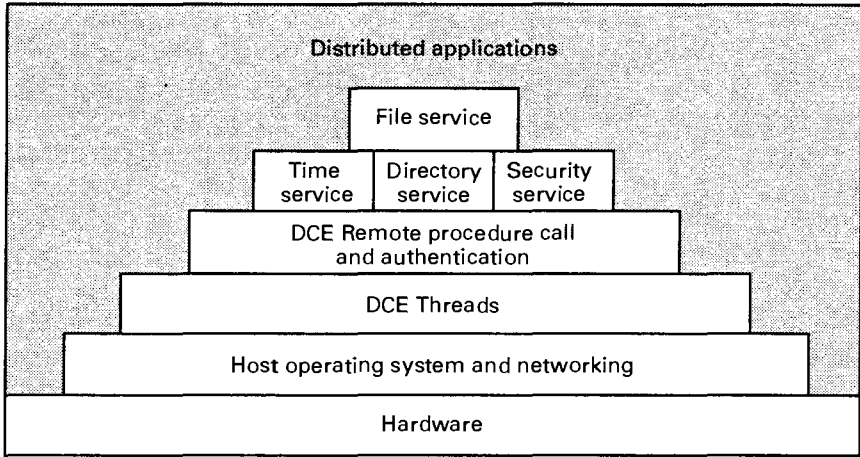
Fig. 10-1. Rough sketch of how the parts of DCE fit together.
