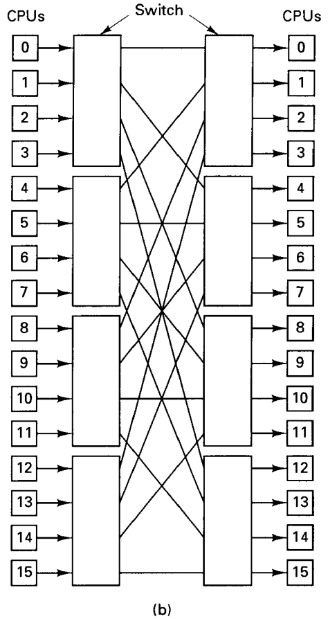
Fig. 6-9. (a) A simplified view of the Cm* system. (b) The BBN Butterfly. The CPUs on the right are the same as those on the left (i.e., the architecture is really a cylinder).
