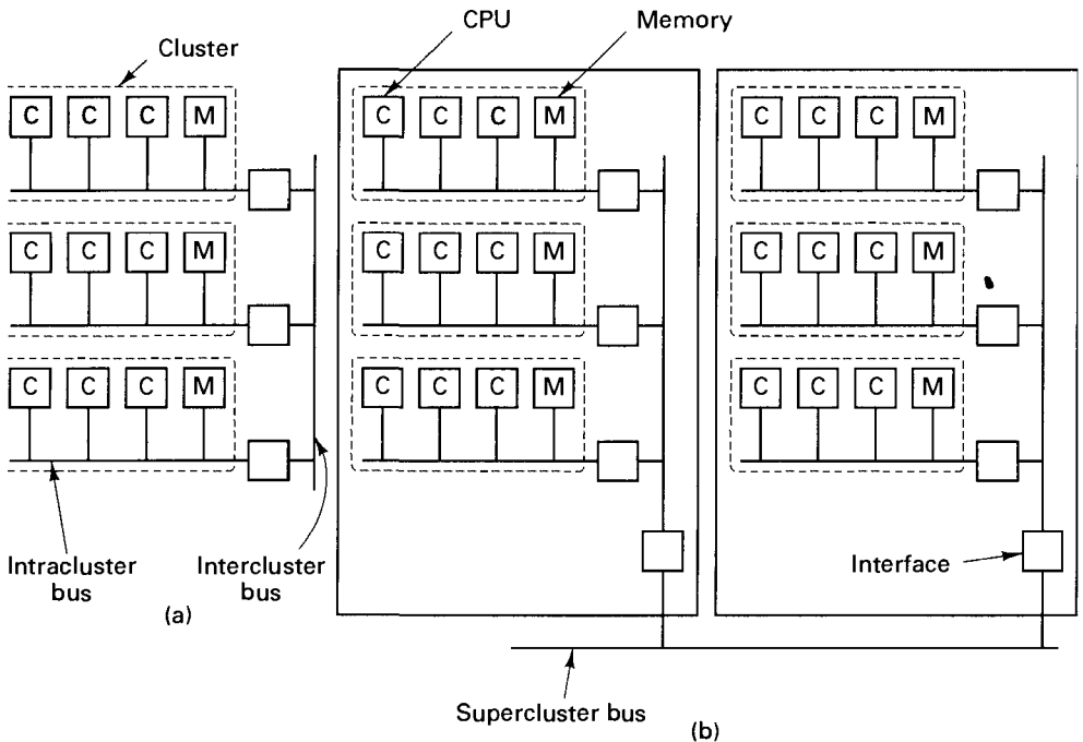
Fig. 6-6. (a) Three clusters connected by an intercluster bus to form one supercluster. (b) Two superclusters connected by a supercluster bus.
