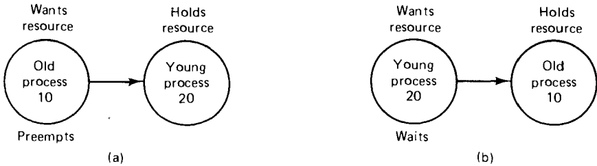
Fig. 3-26. The wound-wait deadlock prevention algorithm.
