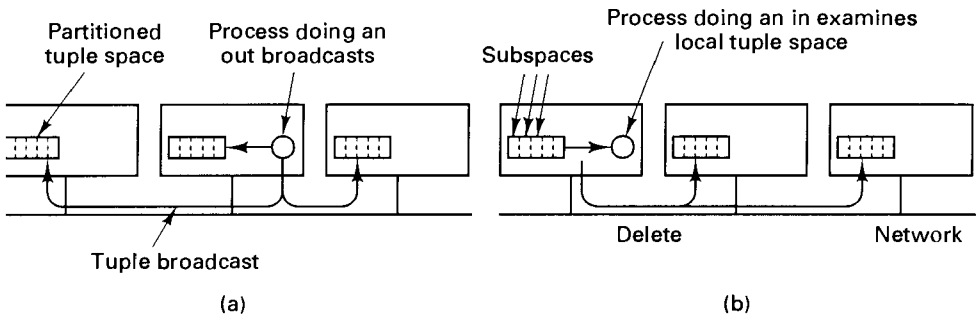
Fig. 6-38. Tuple space can be replicated on all machines. The dotted lines show the partitioning of the tuple space into subspaces. (a) Tuples are broadcast on out . (b) Ins are local, but the deletes must be broadcast.
