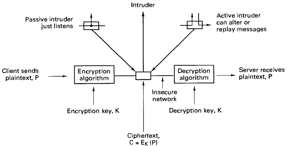
Fig. 10-25. A client sending an encrypted message to a server.
