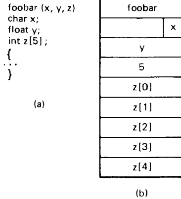
Fig. 2-21. (a) A procedure. (b) The corresponding message.
