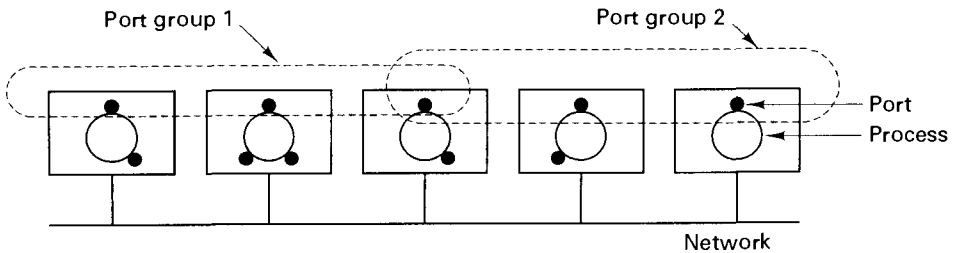
Fig. 9-15. A port may be a member of multiple port groups.
