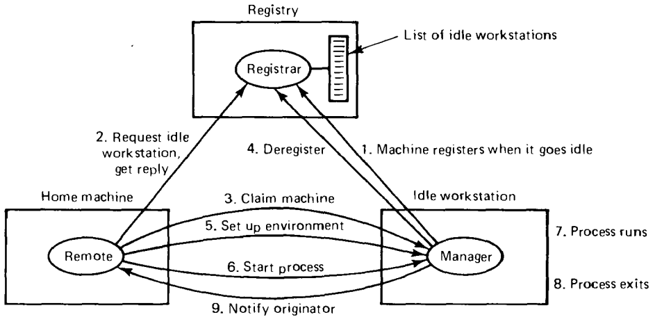
Fig. 4-12. A registry-based algorithm for finding and using idle workstations.
