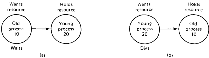
Fig. 3-25. The wait-die deadlock prevention algorithm.
