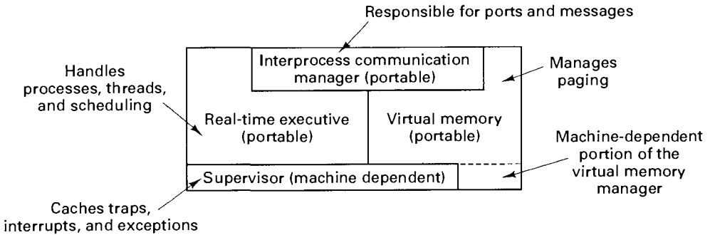
Fig. 9-5. Structure of the Chorus kernel.
