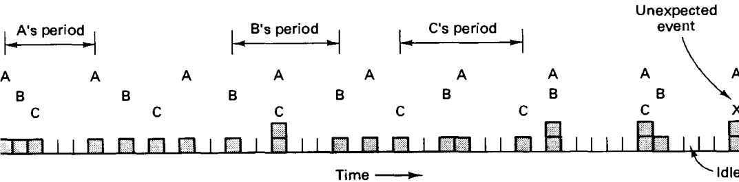
Fig. 4-25. Superposition of three event streams plus one sporadic event.
