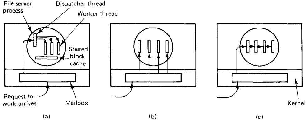
Fig. 4-3. Three organizations of threads in a process. (a) Dispatcher/worker model. (b) Team model. (c) Pipeline model.
