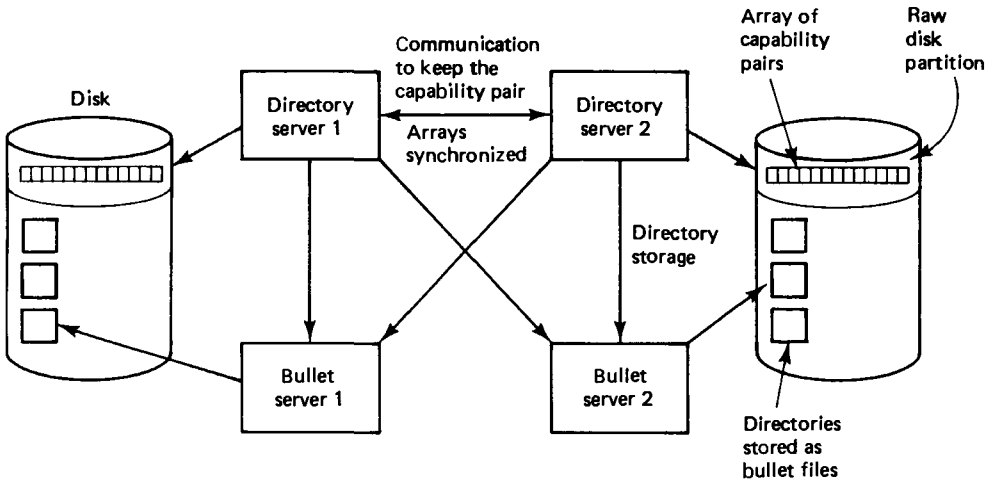
Fig. 7-25. A pair of directory servers. All data are stored twice, on different bullet servers.
