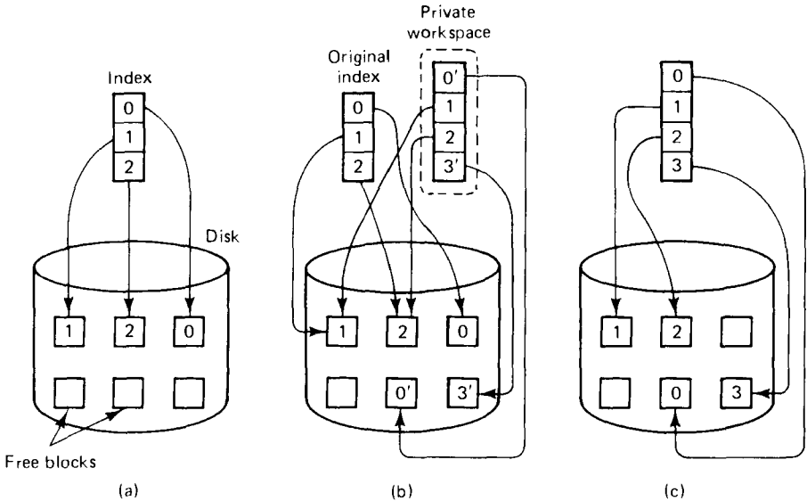
Fig. 3-18. (a) The file index and disk blocks for a three-block file. (b) The situation after a transaction has modified block 0 and appended block 3. (c) After committing.
