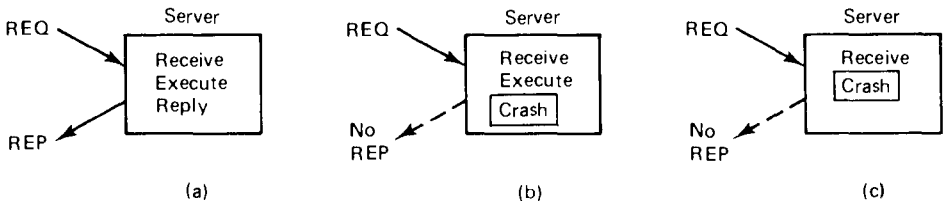
Fig. 2-24. (a) Normal case. (b) Crash after execution. (c) Crash before execution.
