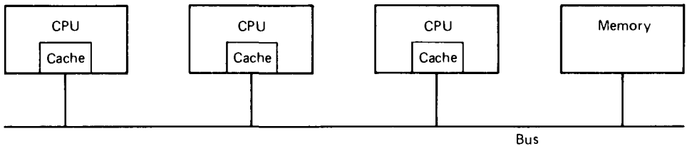
Fig. 1-5. A bus-based multiprocessor.
