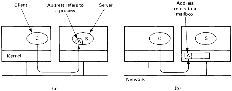
Fig. 2-12. (a) Unbuffered message passing. (b) Buffered message passing.
