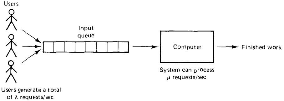
Fig. 4-14. A basic queuing system.
