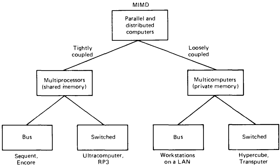
Fig. 1-4. A taxonomy of parallel and distributed computer systems.
