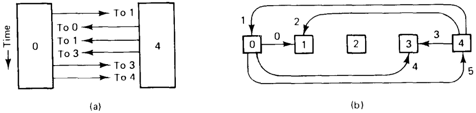
Fig. 2-34. (a) The three messages sent by processes 0 and 4 are interleaved in time. (b) Graphical representation of the six messages, showing the arrival order.
