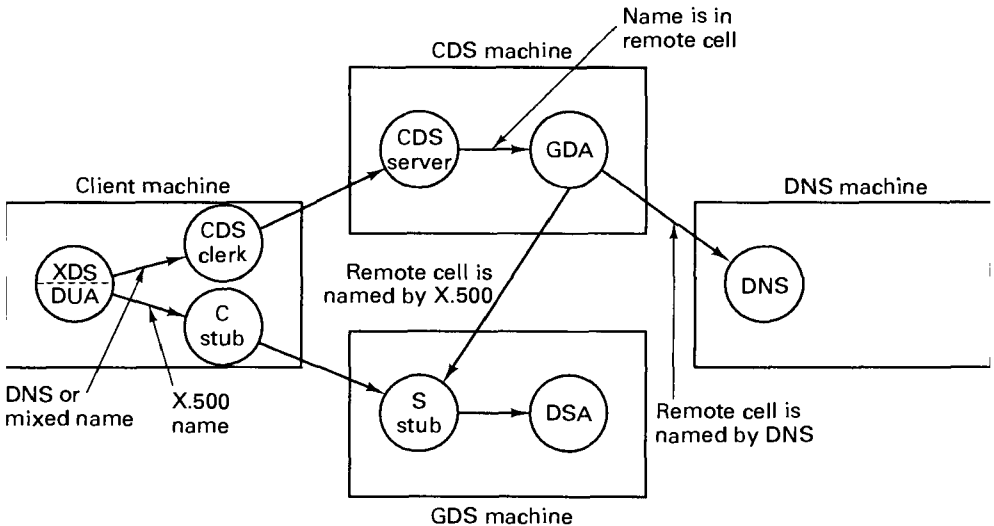
Fig. 10-24. How the servers involved in name lookup invoke one another.
