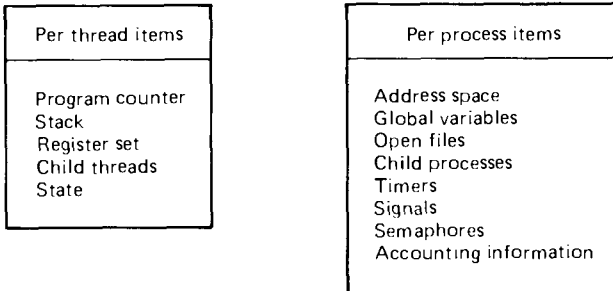
Fig. 4-2. Per thread and per process concepts.
