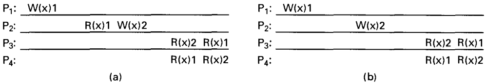
Fig. 6-17. (a) A violation of causal memory. (b) A correct sequence of events in causal memory.
