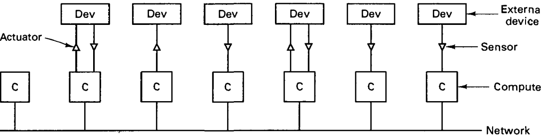
Fig. 4-26. A distributed real-time computer system.
