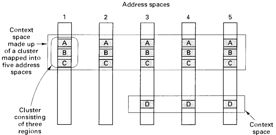
Fig. 9-25. Context spaces and clusters.
