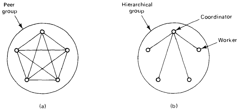
Fig. 2-32. (a) Communication in a peer group. (b) Communication in a simple hierarchical group.
