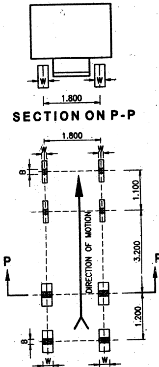
PLAN DRIVING VEHICLE Fig. 2. Class 'A' train of vehicles (Clause 207.1)
