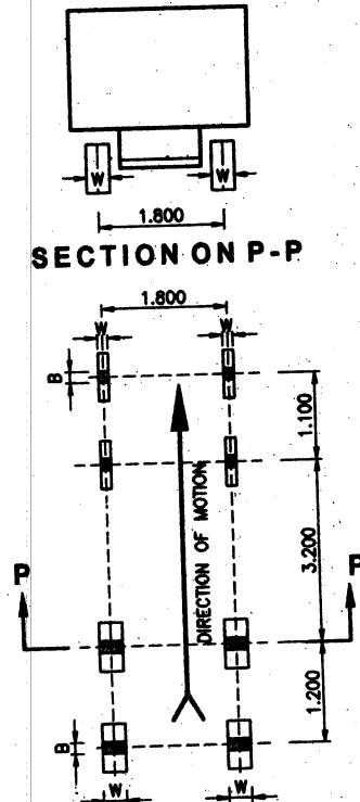
PLAN DRIVING VEHICLE Fig. 3. Class 'B' train of vehicles (Clause 207.1)
