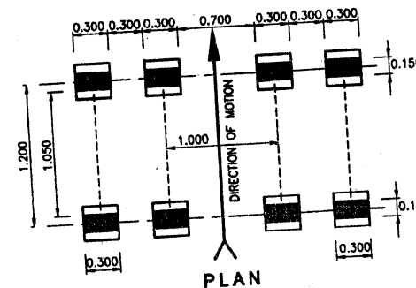
Fig. 1. Class AA tracked and wheeled vehicles (Clause 207.1)
