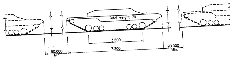
TRACKED VEHICLE
